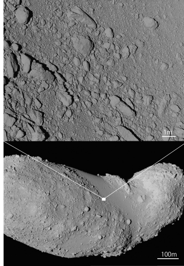
Figure 4: Close-up of the surface of Itokawa.
